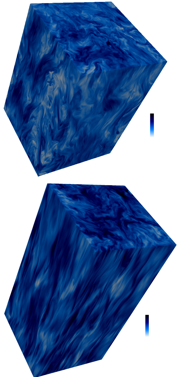
Figure 1: Amplitude squared of magnetic field fluctuations in three-dimensional MHD turbulence subject to a strong mean magnetic field directed perpendicular to the top-side of the volume. The magnitude of the mean magnetic field in the top panel of this figure is 2 times larger than the RMS magnetic fluctuations. The magnitude of the mean magnetic field in the bottom panel is 5 times the RMS magnetic fluctuations. An electrically conducting fluid streams freely in the direction of the magnetic field. As the mean magnetic field is increased, a more elongated simulation box at fixed numerical resolution becomes necessary to deal with the stronger anisotropy of the turbulent eddies. A remarkable increase in the anisotropy of the flow is visible between the simulations. This anisotropy affects not only the direction of the mean magnetic field, but also changes the characteristics of the flow in the perpendicular plane.
