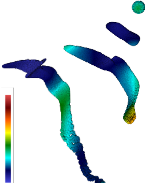
Figure 2: A high-density spherical droplet, represented by 16 thousand Lagrangian particles, dispersing over 10 Kolmogorov time-scales \tau_\eta in anisotropic MHD turbulence with a 2048^3 grid. Particles are colored by the kinetic energy of the fluid.
