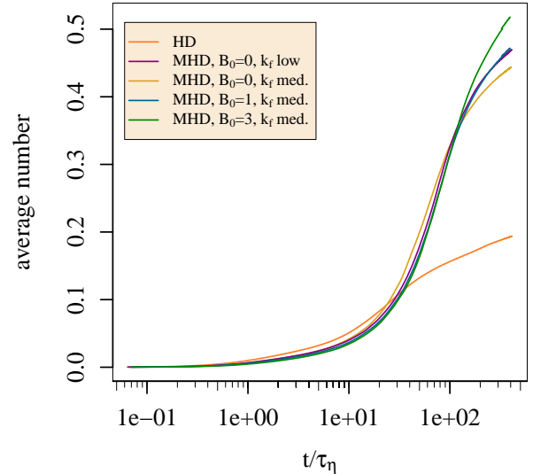
Figure 3: Average number of times that an outer particle of a droplet is engulfed by the group of particles.
