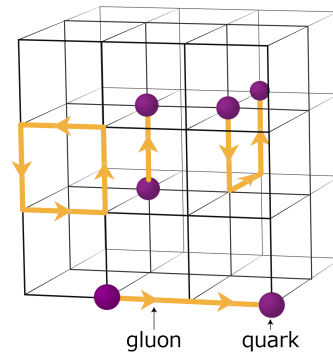
Figure 2: By Guido Cossu. Lattice QCD+QED is a particular formulation of Quantum Chromodynamics and Electrostatics, which is based on the idea to replace the continuous spacetime with a lattice, as in a crystal.
